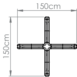
Ultra-plus 59 cm: 48w, cri 80, 3000k ,4816Lm Ultra-plus 59 cm: 90w, cri 80, 3000k ,9160Lm
