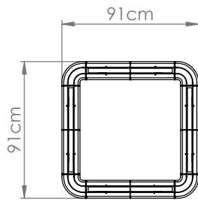
Ultra-square 59 cm: 48w, 80 cri, 3000k ,4816Lm Ultra-square 59 cm: 90w, cri 80, 3000k ,9160Lm
