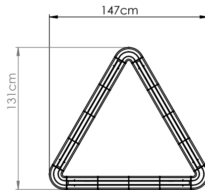
Ultra-triangle 115 cm: 72w, cri 80, 3000k ,7230Lm Ultra-triangle 115 cm: 135w, cri 80, 3000k ,13750Lm
