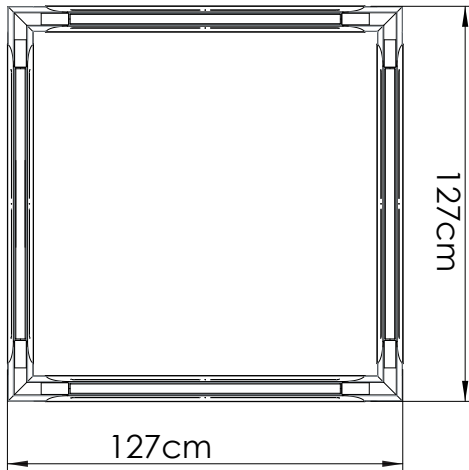
Omega Square 127 cm: 73w, cri 80, 3000k, 7252Lm Omega Square 127 cm: 137w, cri 80, 3000k, 13742Lm
