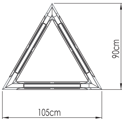
Omega Triangle 105 cm: 36w, cri 80, 3000k, 3615Lm Omega Triangle 105 cm: 68w, cri 80, 3000k, 6870Lm
