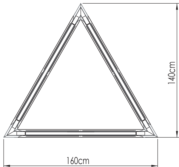
Omega Triangle 160 cm: 72w, cri 80, 3000k, 7225Lm Omega Triangle 160 cm: 137w, cri 80, 3000k, 13740Lm
