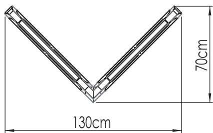
Omega V 130 cm: 24w, cri 80, 3000k, 2400Lm Omega V 130 cm: 45.5w, cri 80, 3000k, 4580Lm
