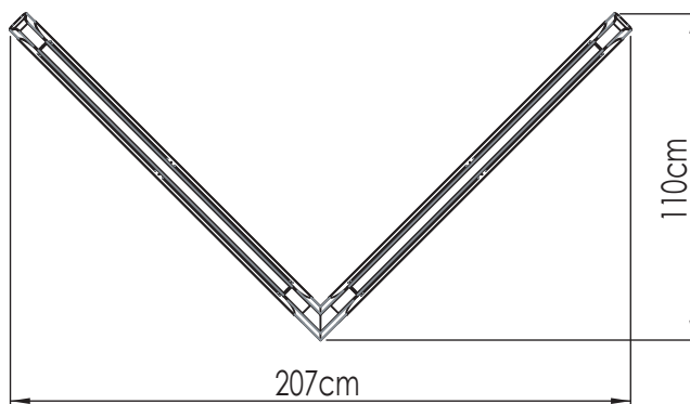
Omega V 207 cm: 48.5w, cri 80, 3000k, 4815Lm Omega V 207 cm: 91w, cri 80, 3000k, 9160Lm
