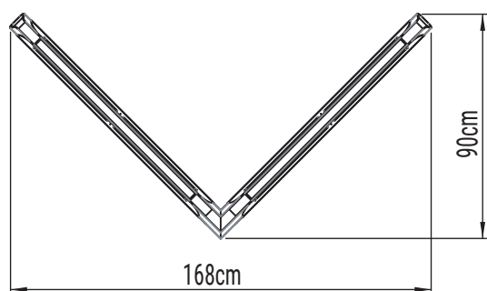
Omega V 168 cm: 36.5w, cri 80, 3000k, 3625Lm Omega V 168 cm: 68.5w, cri 80, 3000k, 6870Lm
