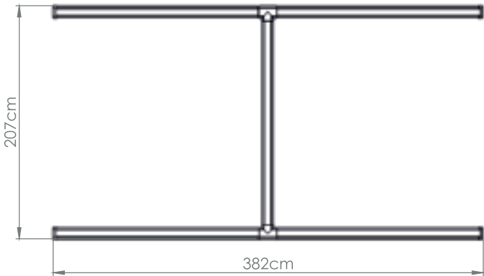
Ladder 185 cm: 181w, cri 80, 3000k, 19600Lm Ladder 185 cm: 370w, cri 80, 3000k, 37220Lm
