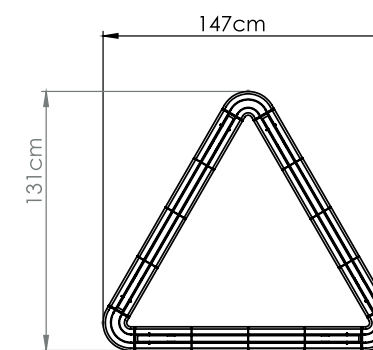
Ultra-triangle 115 cm: 72w, cri 80, 3000k, 7230Lm Ultra-triangle 115 cm: 135w, cri 80, 3000k, 13750Lm
