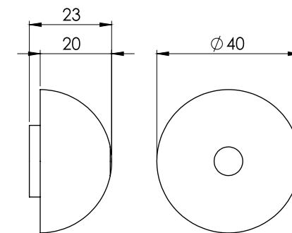
KNITTER WALL DOME - M
