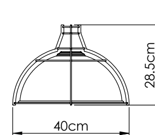
ROYAL BLACKSMITH Dim: Diameter 40 cm
