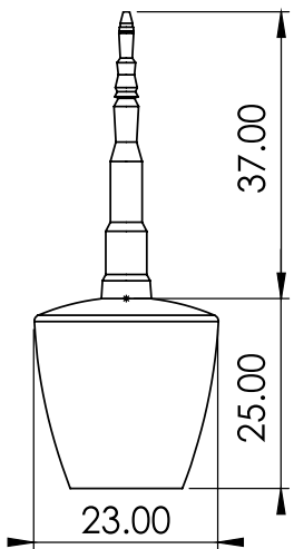
CALLA Dim: Diameter 23 cm H – 25 cm
