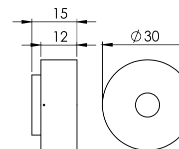
KNITTER WALL CIRCULAR - S
