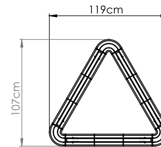
Ultra-triangle 87 cm: 54w, cri 80, 3000k, 5439Lm Ultra-triangle 87 cm: 102w, cri 80, 3000k, 10306Lm
