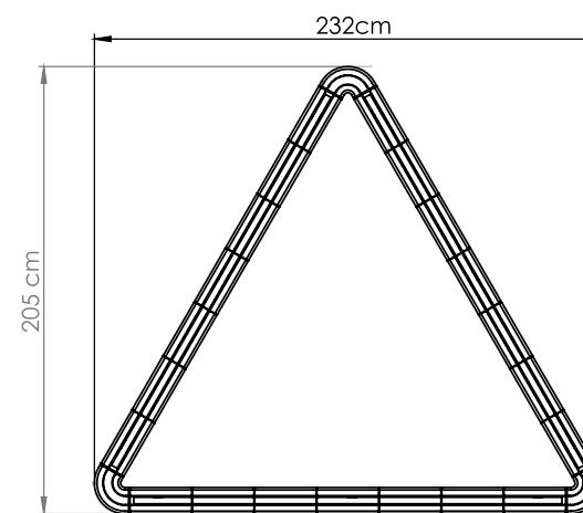
Ultra-triangle 200 cm: 127w, cri 80, 3000k, 12675Lm Ultra-triangle 200 cm: 239w, cri 80, 3000k, 24060Lm
