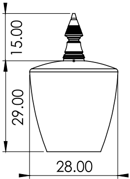
CALLA Dim: Diameter 28 cm H – 29 cm
