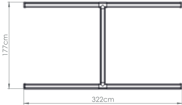
Ladder 165 cm: 153w, cri 80, 3000k, 15855Lm Ladder 165 cm: 313w, cri 80, 3000k, 30050Lm
